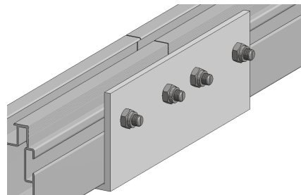
COUPLING - JOIST 75
